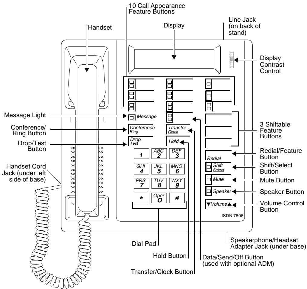
Figure 17-2. The 7506 Asynchronous Data Modular Display Terminal
